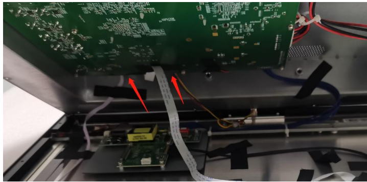
Step 20: Connect the keyboard cable back.
