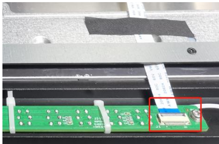
Step 21: Use tape to fix the ribbon cable.
