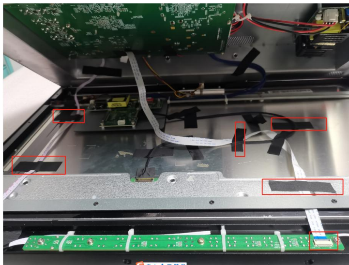
Step 22: Connect the screen cable back.
