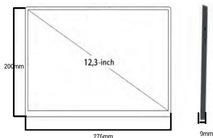
12.3" portable monitor
